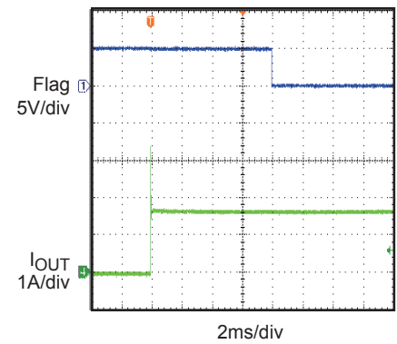
1\Omega Load Connected to Enabled Device
