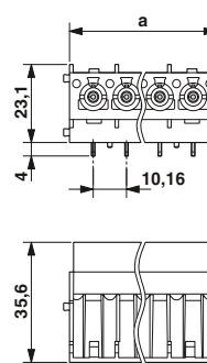
Dimensional drawing: VC-AML...
