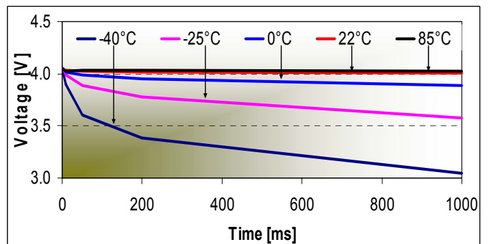
Pulse capability of 0.5 A at several temperatures
