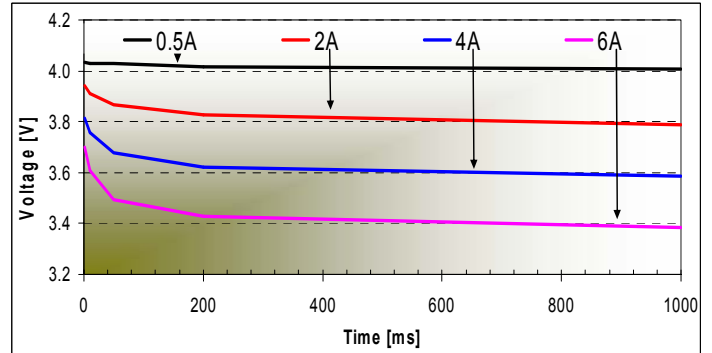
Pulse capability at RT
