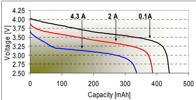
Discharge capability at RT
