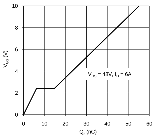
Figure 12. Gate Charge
