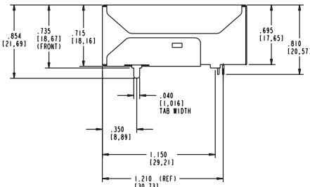
Digi Connect ME® - Side
