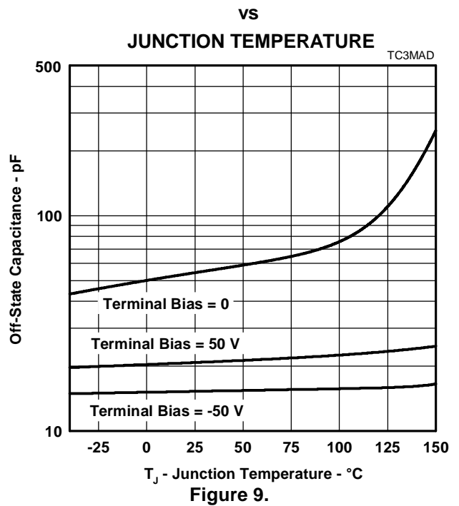
OFF-STATE CAPACITANCE
