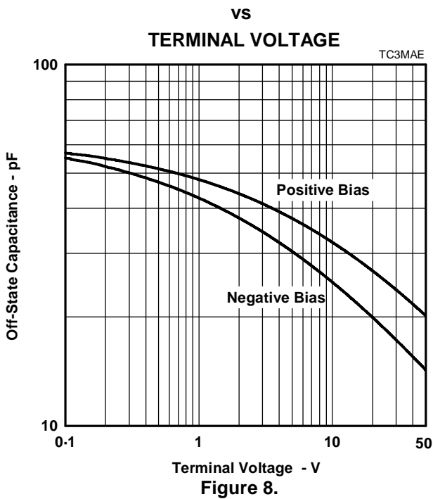
OFF-STATE CAPACITANCE
