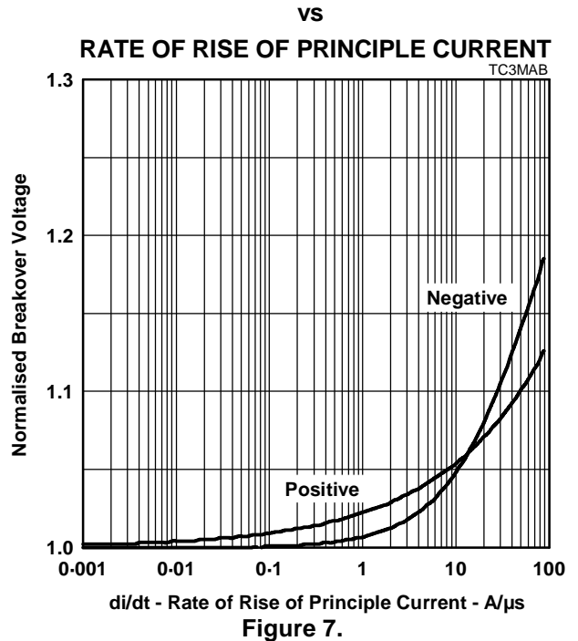
NORMALISED BREAKOVER VOLTAGE
