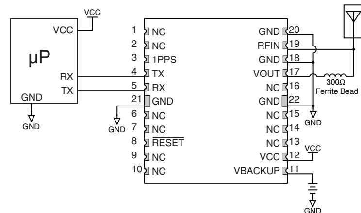
Figure 38: Circuit Using the GM Series Module with a an Active Antenna
