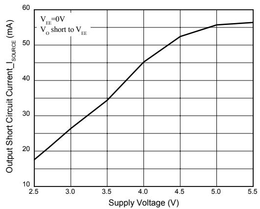
Figure 7. Output Short Circuit Current vs. Supply Voltage
