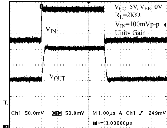
Figure 21. Non-Inverting Input Small Signal Pulse Response
