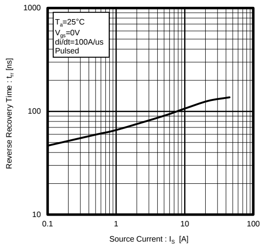
Fig.13 Reverse Recovery Time vs. Source Current
