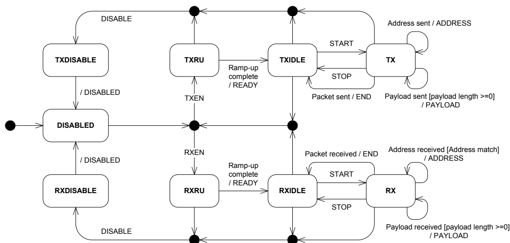
Figure 34: Radio states
