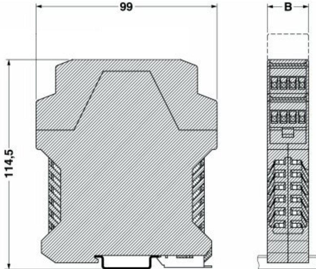
Dimensioned drawing
