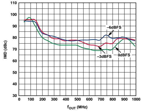
Figure 98. IMD vs. f_{OUT} over Digital Full Scale
