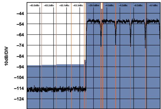
Figure 143. Low Band Narrow-Band ACLR
