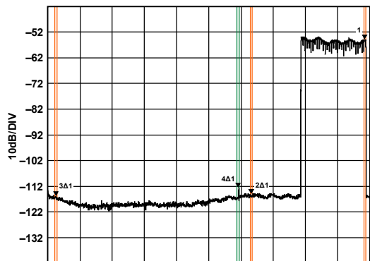
Figure 141. Mid Band Wideband ACLR
