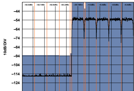
Figure 144. Mid Band Narrow-Band ACLR (Worse Side)
