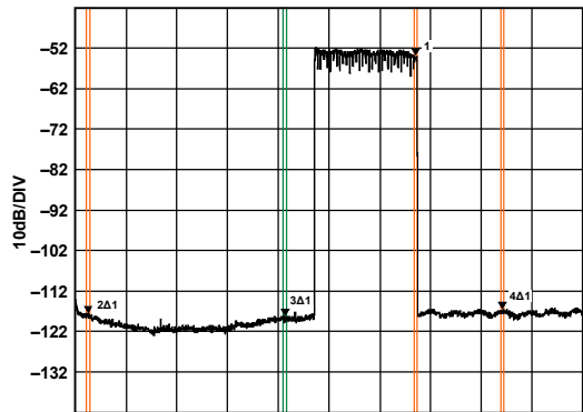
Figure 140. Low Band Wideband ACLR
