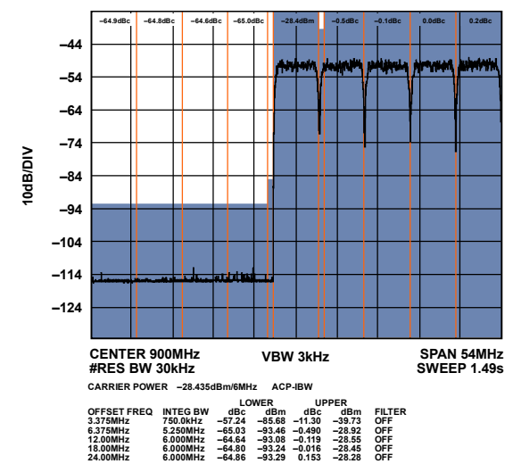
Figure 139. High Band Narrow-Band ACLR
