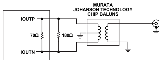
Figure 185. Lowest Cost and Size Configuration for Narrow RF Band Operation
