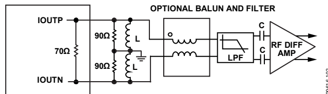
Figure 183. Interfacing the DAC Output to the Self-Biased Differential Gain Stage
