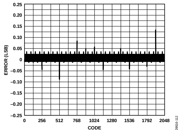
Figure 12. Typical DNL, 10 mA at 25^\circ\text{C}
