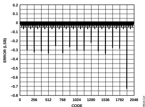
Figure 14. Typical DNL, 30 mA at 25^\circ\text{C}
