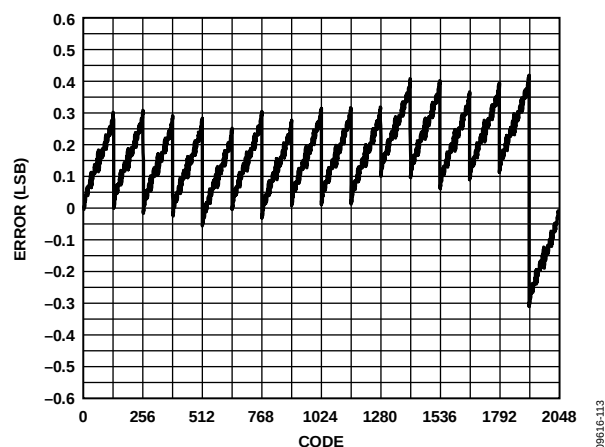
Figure 13. Typical INL, 30 mA at 25^\circ\text{C}
