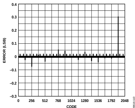
Figure 10. Typical DNL, 20 mA at 25^\circ\text{C}
