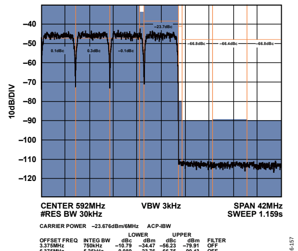
Figure 58. Mid Band Narrow-Band ACLR (Worse Side)
