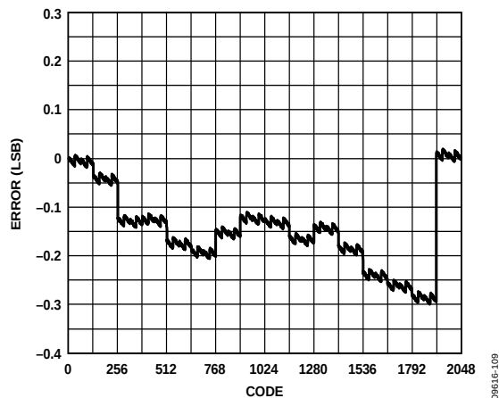
Figure 9. Typical INL, 20 mA at 25^\circ\text{C}
