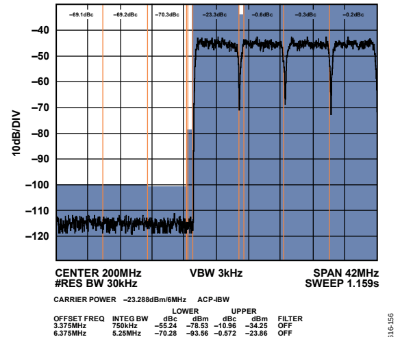
Figure 57. Low Band Narrow-Band ACLR (Worse Side)
