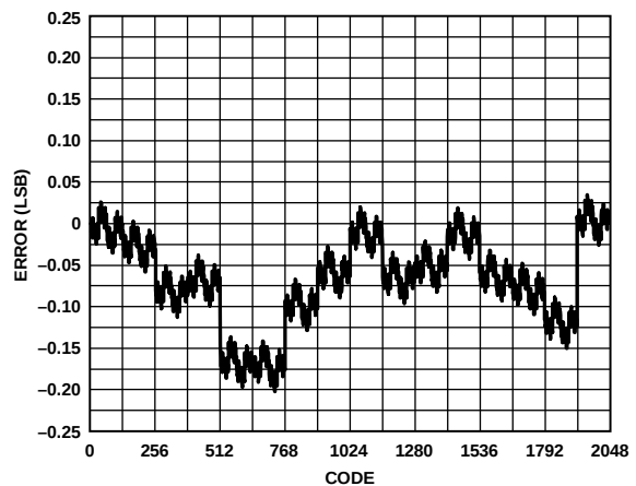
Figure 11. Typical INL, 10 mA at 25^\circ\text{C}
