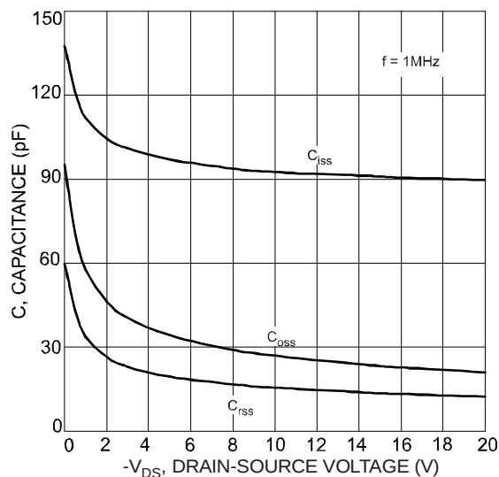
Fig. 10 Typical Capacitance
