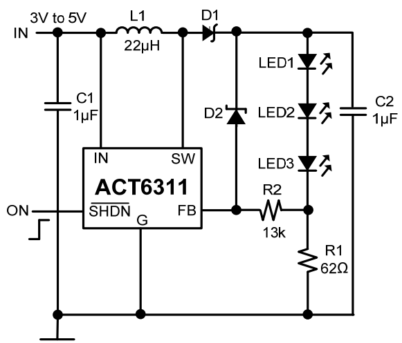
Figure 9: Open-Circuit Protection
