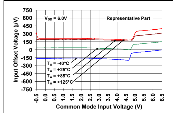
FIGURE 2-4: Input Offset Voltage vs. Common Mode Input Voltage with V_{DD} = 6.0\text{V} .
