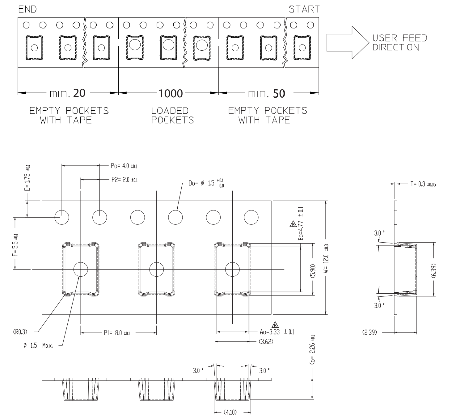
Figure 19. Emitter pocket tape packaging.
