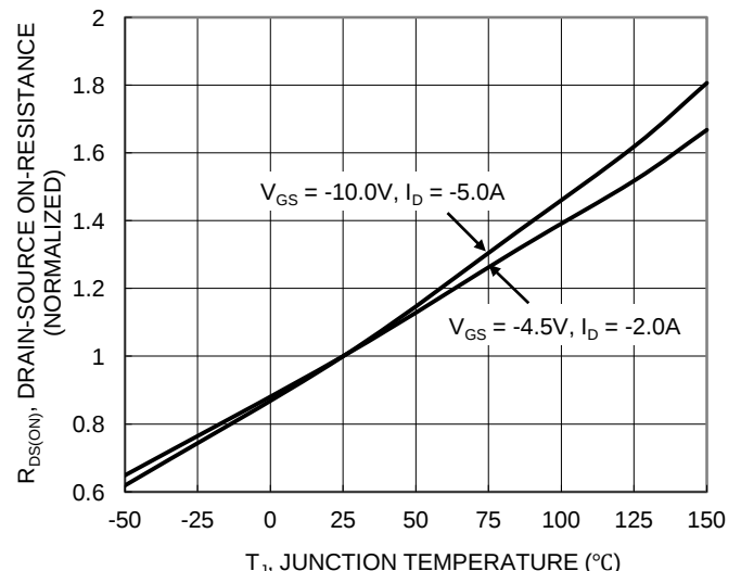
Figure 19. On-Resistance Variation with Temperature
