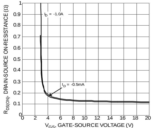
Figure 17 Typical Drain-Source On-Resistance vs. Gate-Source Voltage
