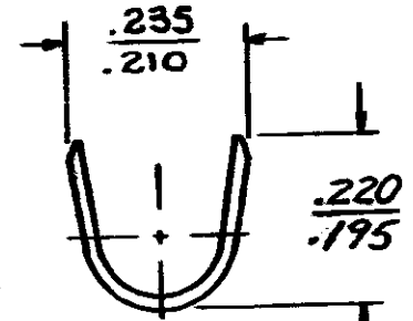
SECT B-B
