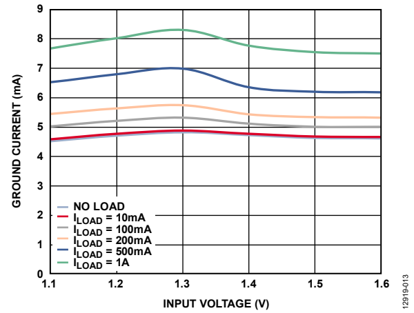
Figure 13. Ground Current vs. Input Voltage (in Dropout), V_{OUT} = 1.3\text{ V}
