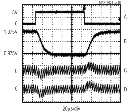
VID CODE CHANGE ( \overline{SLOW} = GND )
