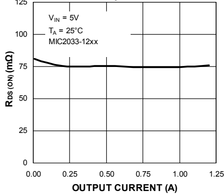
RDS(ON) vs. Output Current
