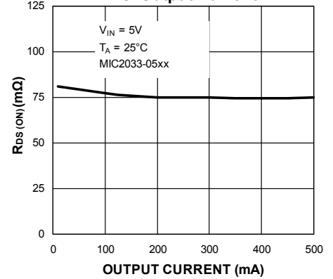
RDS(ON) vs. Output Current
