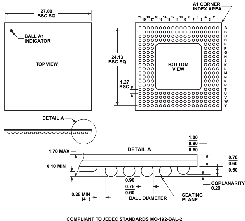
Figure 52. 256-Ball Ball Grid Array, Thermally Enhanced [BGA_ED] (BP-256) Dimension shown in millimeters
