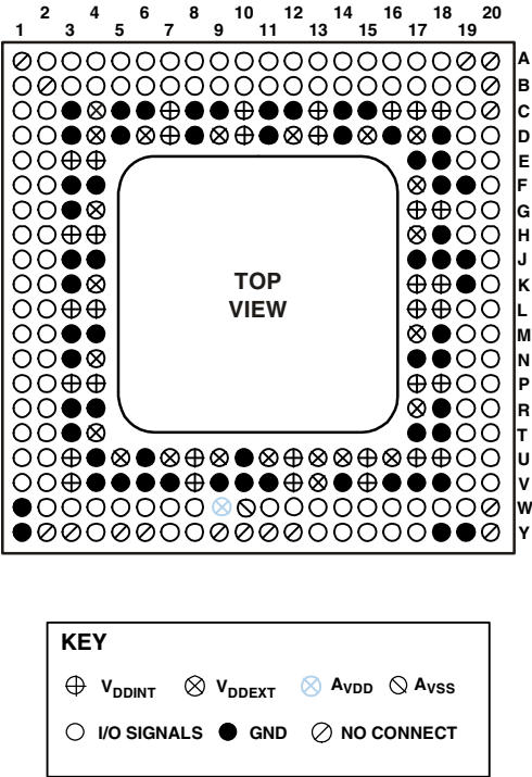
Figure 50. 256-Ball BGA_ED Ball Configuration (Top View)
