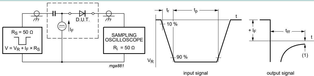
Fig. 13. Reverse recovery time: test circuit and waveforms
