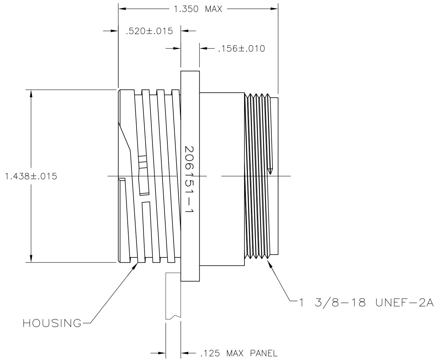
DETAIL A
