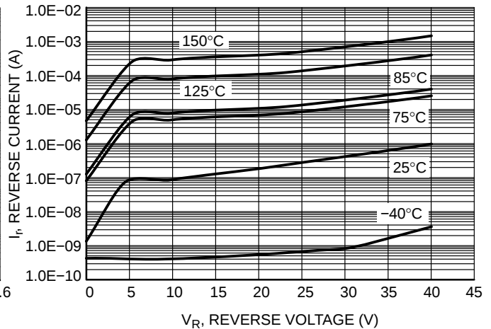
Figure 2. Leakage Current
