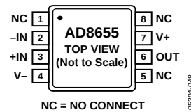
Figure 1. AD8655 8-Lead MSOP (RM-8) 8-Lead SOIC (R-8)
