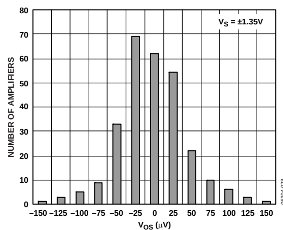
Figure 31. Input Offset Voltage Distribution
