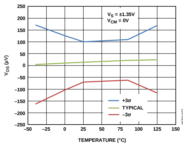
Figure 32. Input Offset Voltage vs. Temperature
