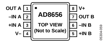
Figure 2. AD8656 8-Lead MSOP (RM-8) 8-Lead SOIC (R-8)
