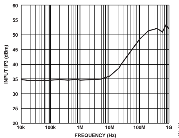
Figure 16. Input IP3 vs. Frequency (Low Frequency Detail)
