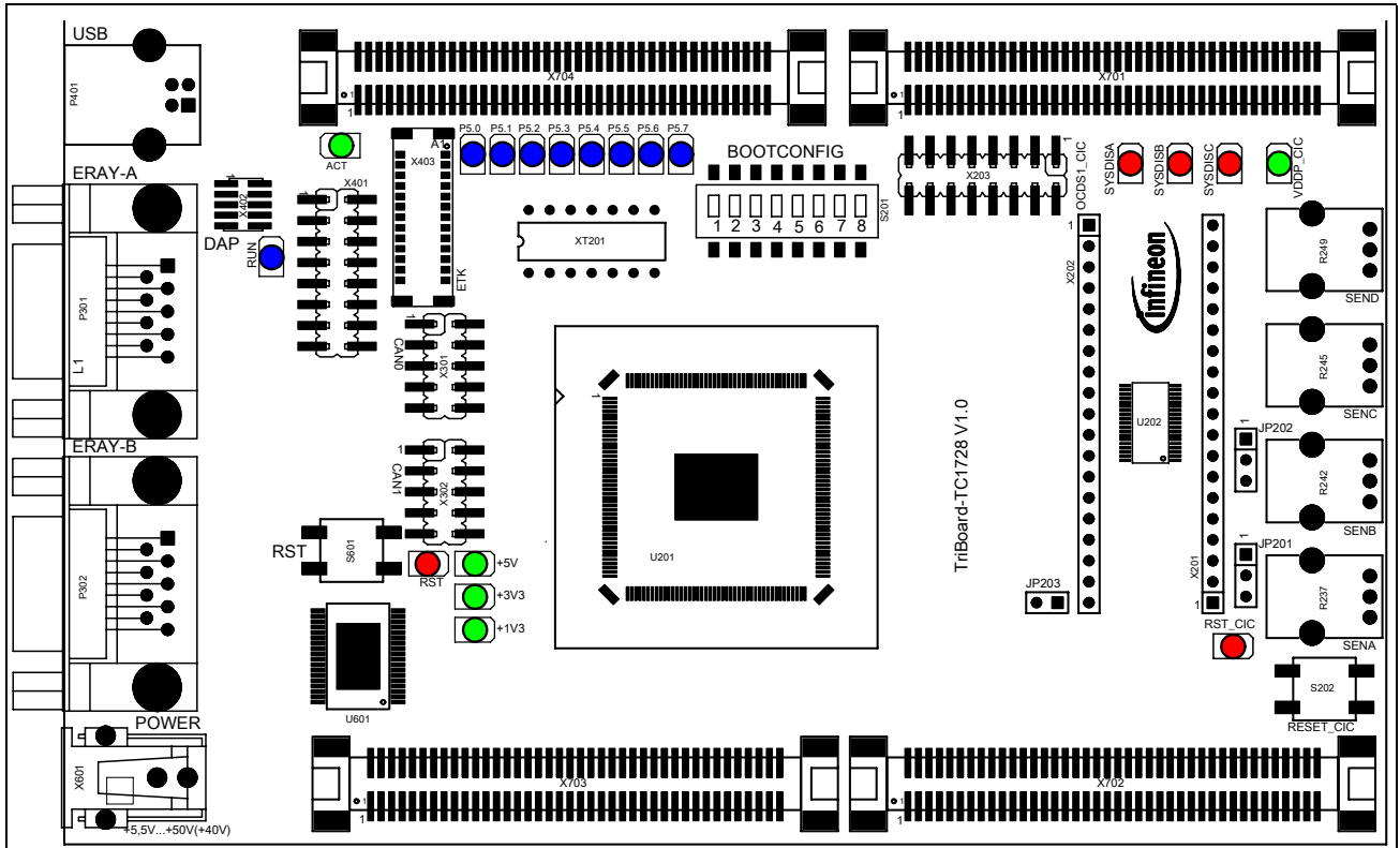
Figure 2-2 TriBoard TC1728 V1.0 Placement
