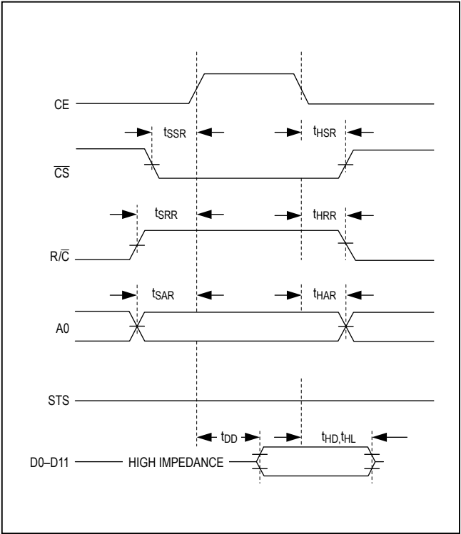
Figure 5. Read Timing
