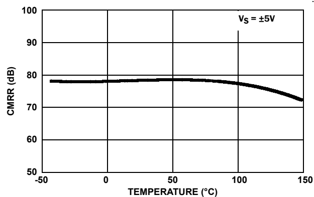
FIGURE 8. CMRR vs TEMPERATURE
