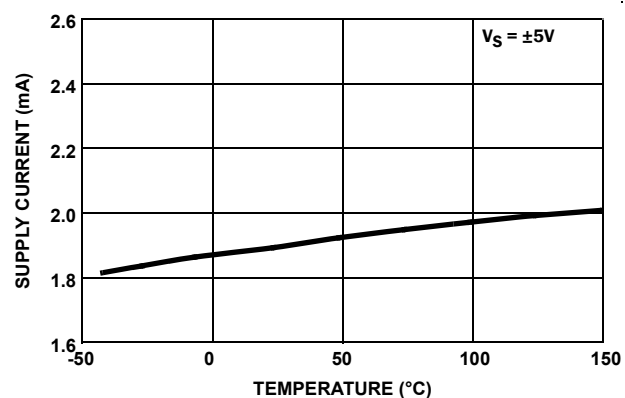
FIGURE 10. SUPPLY CURRENT vs TEMPERATURE
