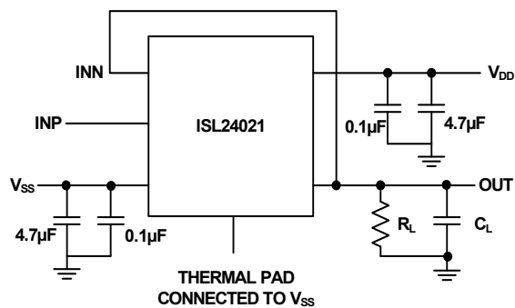
FIGURE 22. TEST CIRCUIT
