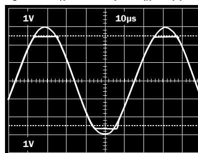
FIGURE 23. OPERATION WITH BEYOND-THE-RAILS INPUT
