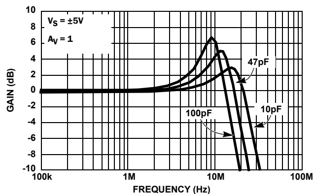
FIGURE 14. FREQUENCY RESPONSE FOR VARIOUS C_L
