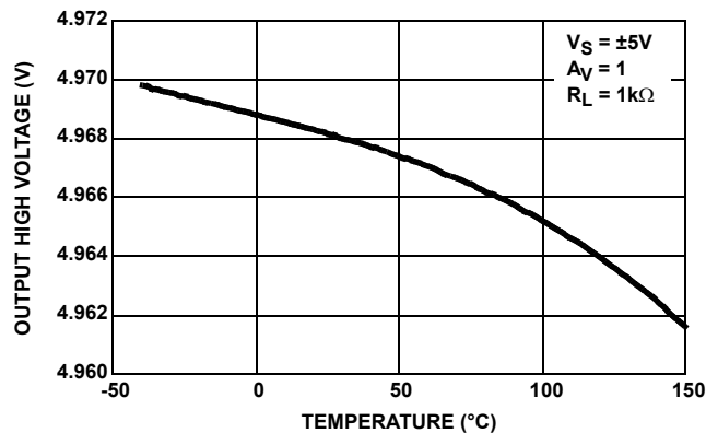
FIGURE 4. OUTPUT HIGH VOLTAGE vs TEMPERATURE
