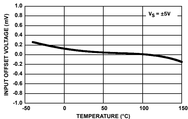
FIGURE 2. INPUT OFFSET VOLTAGE vs TEMPERATURE
