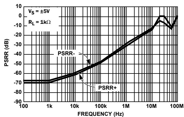
FIGURE 18. PSRR vs FREQUENCY
