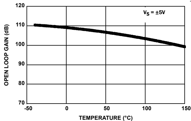
FIGURE 6. OPEN-LOOP GAIN vs TEMPERATURE
