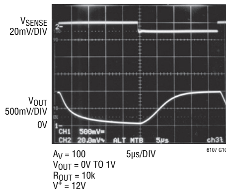
Step Response 0mV to 10mV (RIN = 100Ω)
