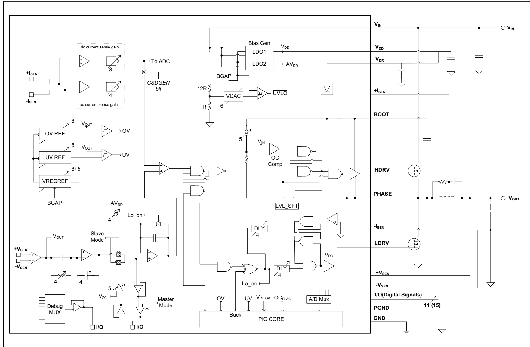
MCP19110/11
