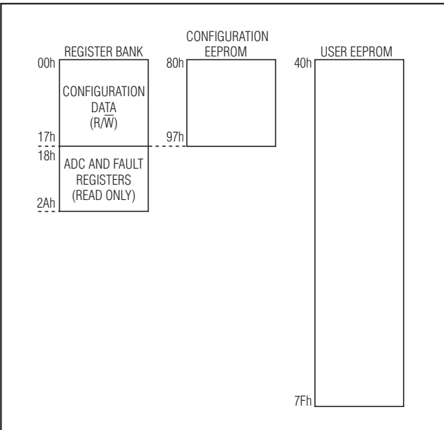
Figure 5. Memory Map
