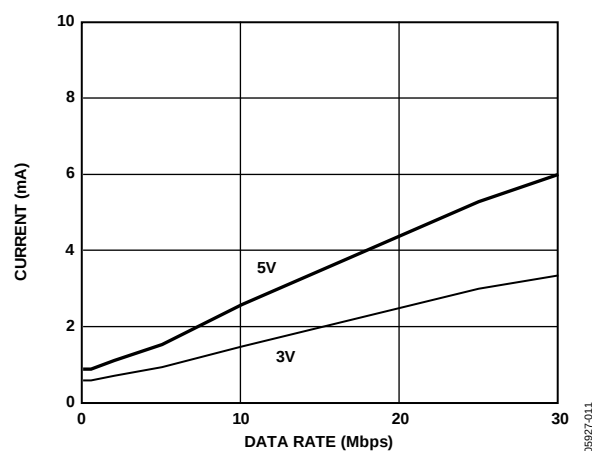
Figure 11. Typical ADuM3201 I_{DD1} or I_{DD2} Supply Current vs. Data Rate for 5 V and 3 V Operation
