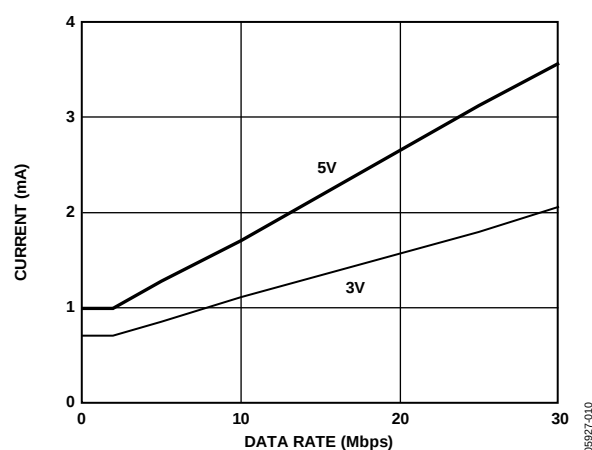
Figure 10. Typical ADuM3200 I_{DD2} Supply Current vs. Data Rate for 5 V and 3 V Operation
