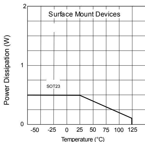
Power Derating
