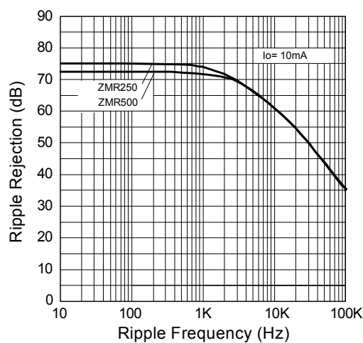
Ripple Rejection v Ripple Frequency
