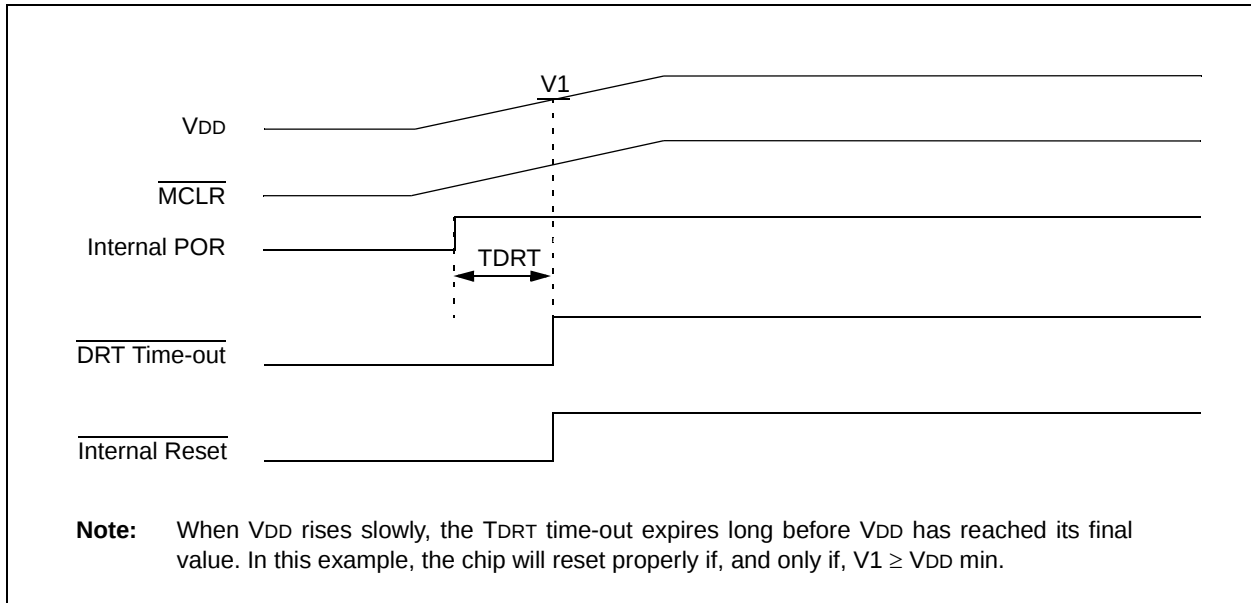
FIGURE 8-10: TIME-OUT SEQUENCE ON POWER-UP ( \overline{\text{MCLR}} TIED TO V_{DD} ): SLOW V_{DD} RISE TIME
