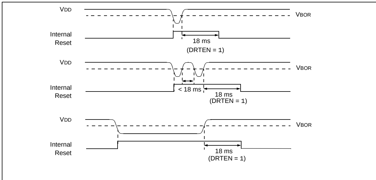
FIGURE 8-13: BROWN-OUT SITUATIONS
