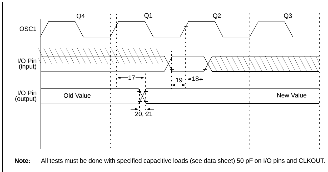
FIGURE 15-5: I/O TIMING
