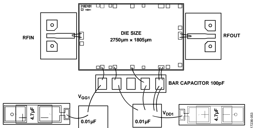
Figure 53. Assembly Diagram
