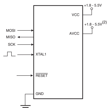
Figure 27-10. Serial Programming and Verify (1)
