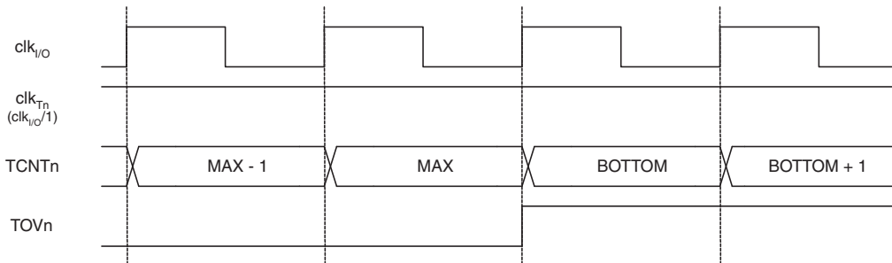
Figure 1. Timer/Counter Timing Diagram, no Prescaling
