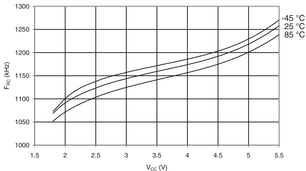
Figure 29-41. ATmega329P: Watchdog Oscillator Frequency vs. V_{CC}
