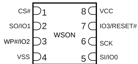
Figure 38. 8-Connector Package (WSO6), Top View
