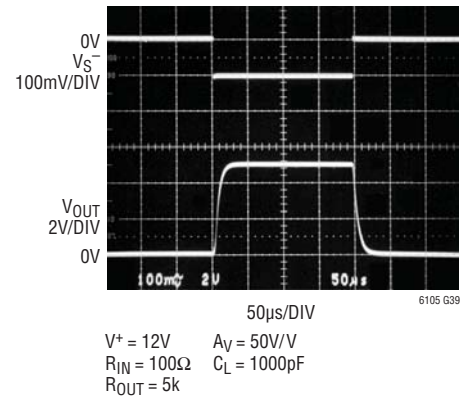
Step Response V_{SENSE} = 0V to 100mV , C_L = 1000pF , V_{S^+} = 0V
