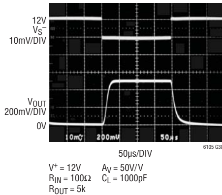
Step Response V_{SENSE} = 0V to 10mV , C_L = 1000pF , V_{S^+} = 12V
