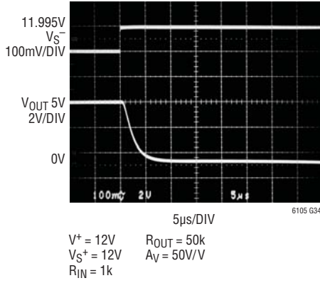
Step Response V_{SENSE} = 100mV to 5mV
