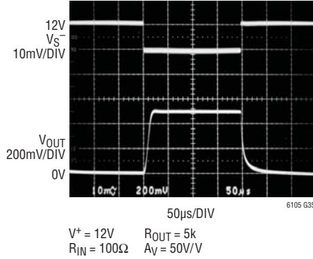
Step Response V_{SENSE} = 0V to 10mV , V_{S^+} = 12V
