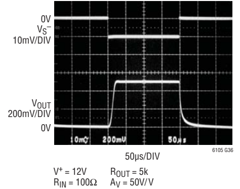
Step Response V_{SENSE} = 0V to 10mV , V_{S^+} = 0V
