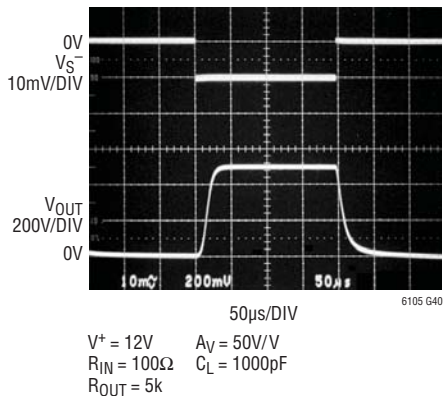
Step Response V_{SENSE} = 0V to 10mV , C_L = 1000pF , V_{S^+} = 0V
