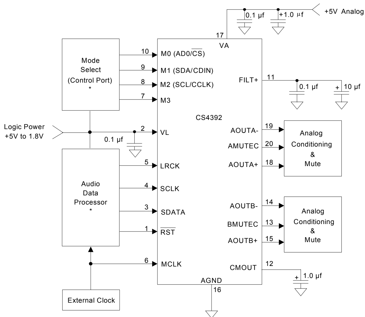
Figure 1. Typical Connection Diagram - PCM Mode
