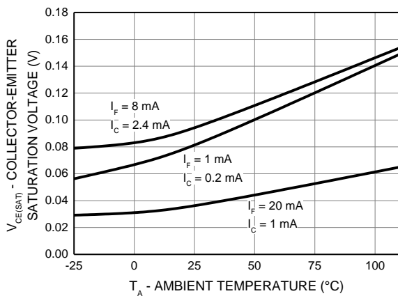
Figure 11. Collector-Emitter Saturation Voltage vs. Ambient Temperature
