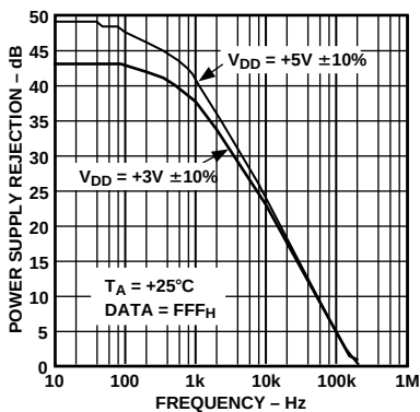
Figure 8. Power Supply Rejection vs. Frequency
