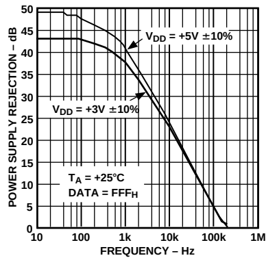
Figure 8. Power Supply Rejection vs. Frequency
